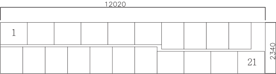
40' CONTAINER(TOP VIEW)
