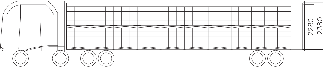
40' CONTAINER(SIDE VIEW)
