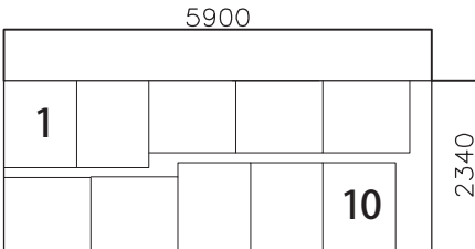
20' CONTAINER(TOP VIEW)
